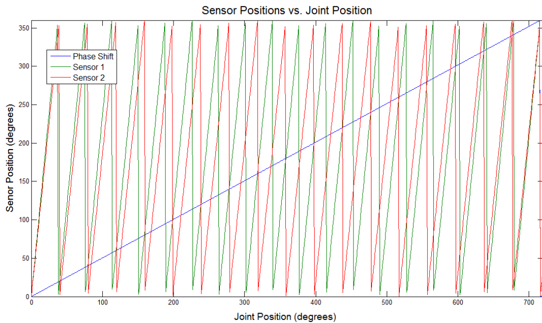
Figure 4.7 Shoulder flexion joint sensor positions and phase shift between the sensors
