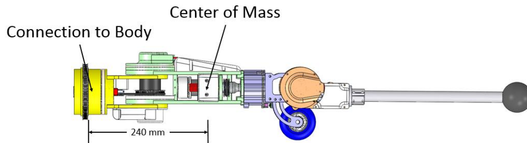
Figure 3.29 uBot-7 arm center of mass location
